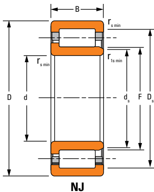
NJ
