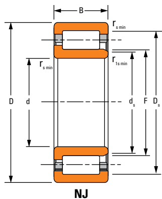
NJ
