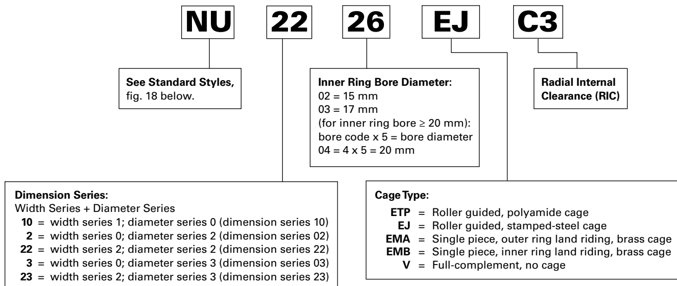
Fig. 17. Metric ISO radial cylindrical roller bearings nomenclature.
