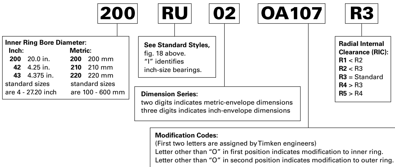
Fig. 19. ABMA radial cylindrical roller bearings nomenclature.
