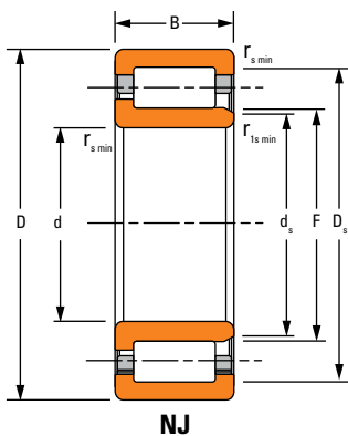
NJ
