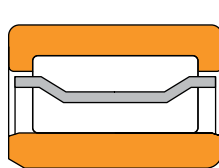
Fig. 3. S-type cage.
