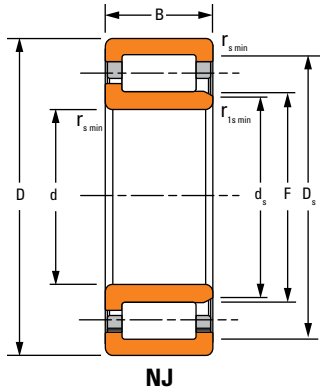
NJ
