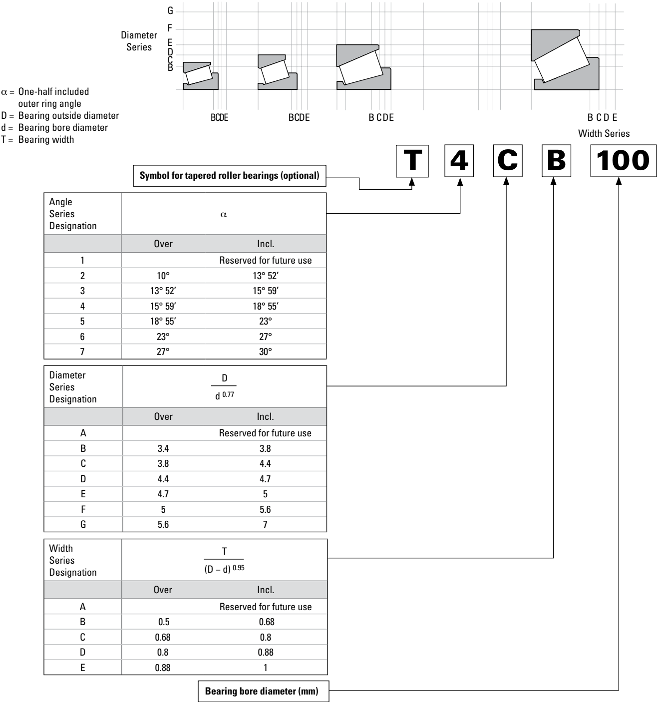
Fig. 32. ISO 355 part-numbering system.
