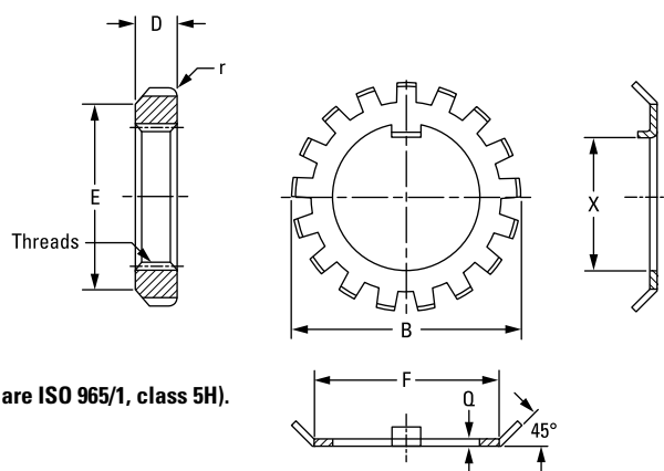
Fig. 50. Lockwashers.
