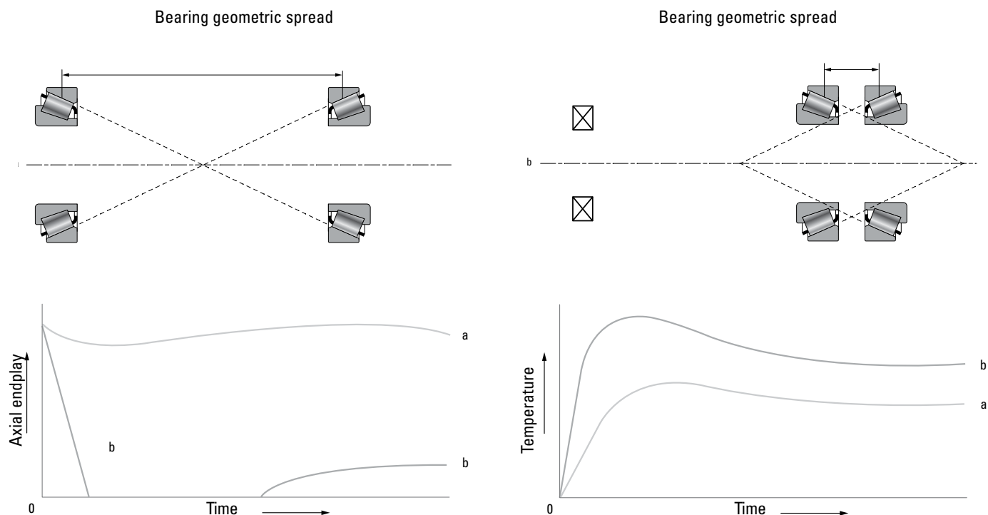
Fig. 95. Evolution of the spindle system setting and temperature during the transient period:
