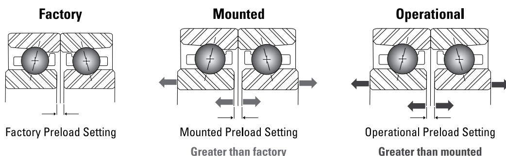
Fig. 23. Preload settings.
