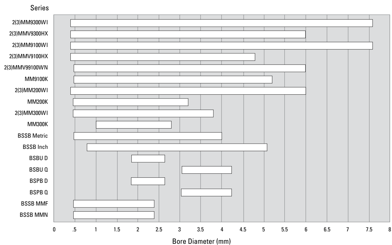
Fig. 136. Bore diameters.
