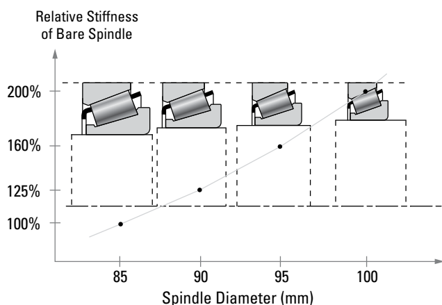
Fig. 26. Influence of spindle diameter on its stiffness for different tapered roller bearing sections within same envelope (85 mm bore taken as reference).
