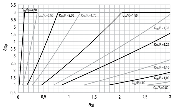
Fig. 52. Low load factor ( a_{3p} ) vs. lubricant life factor ( a_{3l} ) and C_{90}/P_r ratio.
