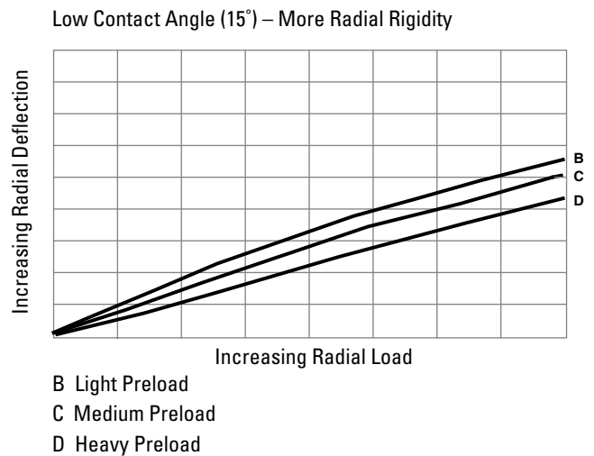
Fig. 19. Effect of contact angle on radial deflection.
