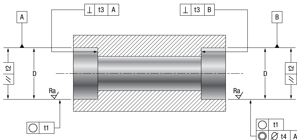
Fig. 70. Housing Tolerances.
