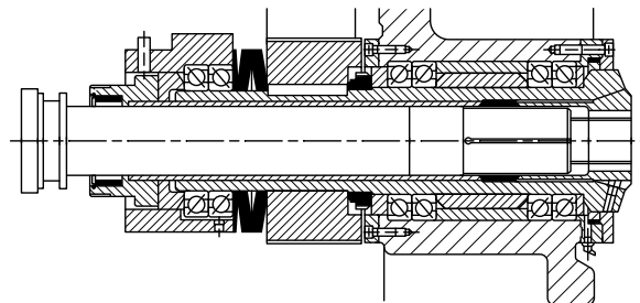
Fig. 130. Single-bar machine.
