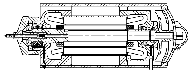
Fig. 134. High-speed motorized router.
