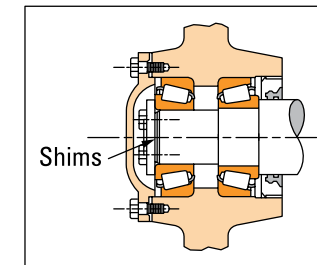
Figure 23. End Plate
