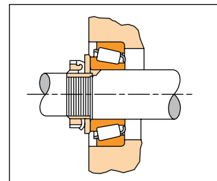
Figure 21. Locknut
