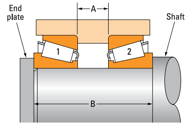
Figure 7. Machine Assembly
