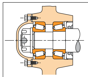
Figure 20. Slotted Nut
