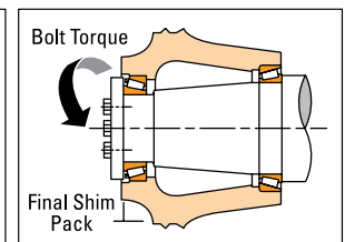
Figure 18. Assembly Complete
