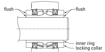
Line up collars with inner ring
