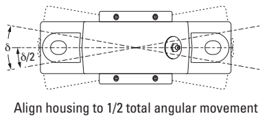
Align housing to 1/2 total angular movement
