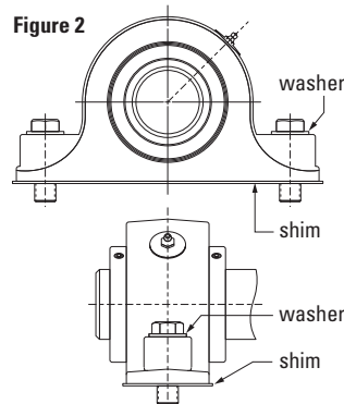
Use washers and full shims
