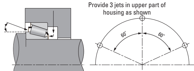
Fig. 59. Cooling jets in top part of the housing for speed above 25 m/s (4920 fpm).
