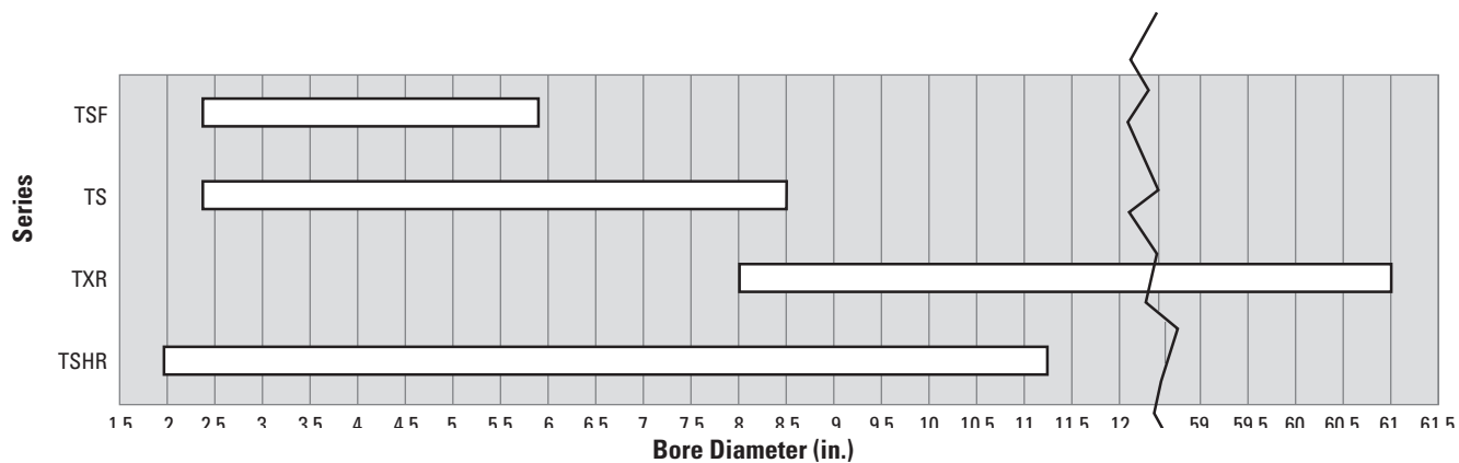
Fig. 109. Bore diameters.
