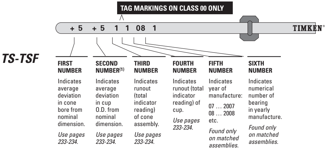
Fig. 102. Inch system precision bearing tag markings.
