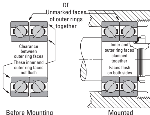
Fig. 84. Face-to-face bearing assemblies before and after mounting.
