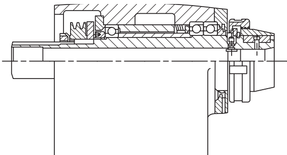
Fig. 133. Super precision lathe headstock.
