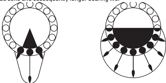
Fig. 46. Bearing load zones and rolling element-raceway contact loading.
