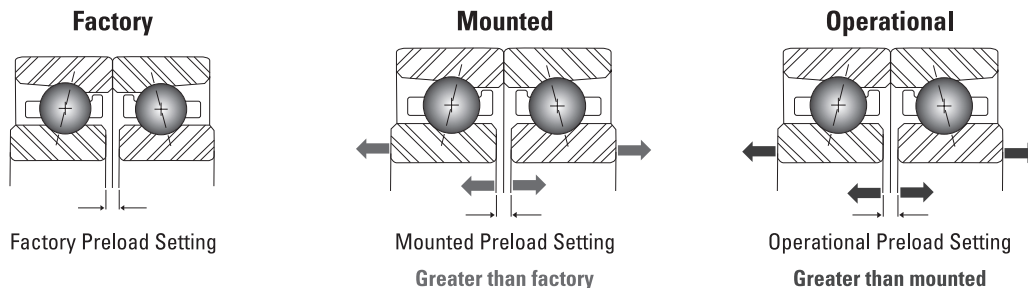
Fig. 23. Preload settings.
