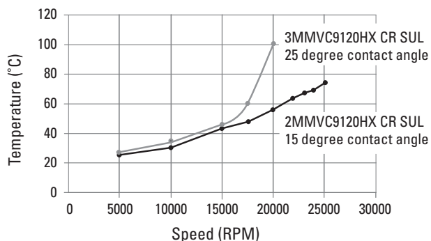
Fig 17. Effect of contact angle on temperature.
