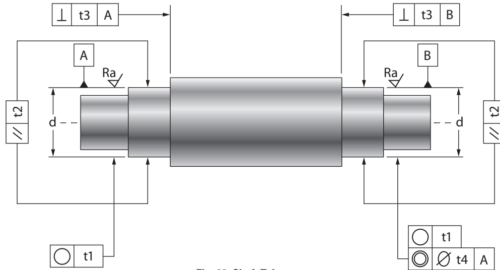
Fig. 69. Shaft Tolerances.
