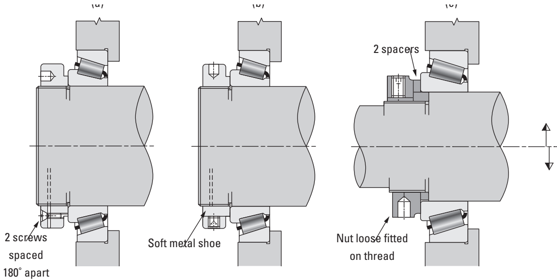
Fig. 71. Locking devices.
