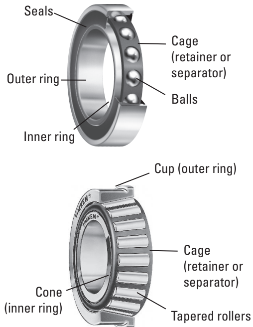
Fig. 2. Bearing components.
