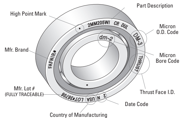
Fig. 121. Super precision markings.
