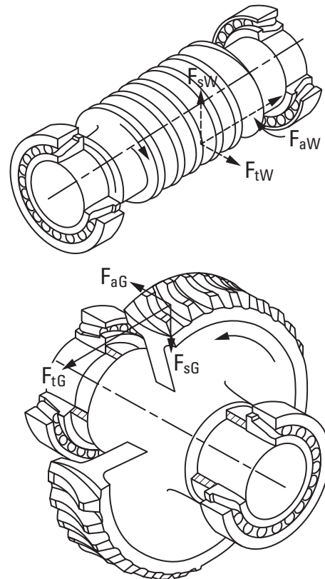
Fig. 42. Straight worm gearing.
