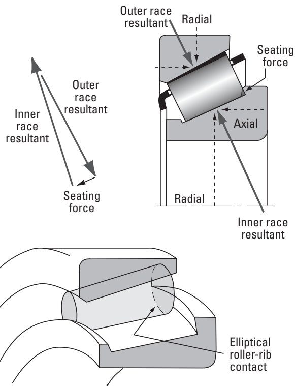
Fig. 10. Small seating force from the inner race rib keeps rollers aligned on the raceway.
