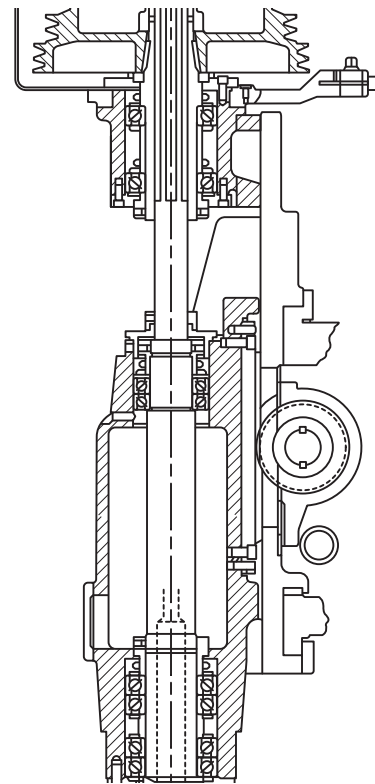
Fig. 135. Precision vertical milling spindle.
