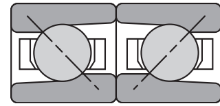
Face-to-Face DF
