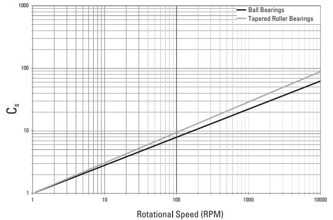
Fig. 49. Speed factor ( C_s ) vs. rotational speed.
