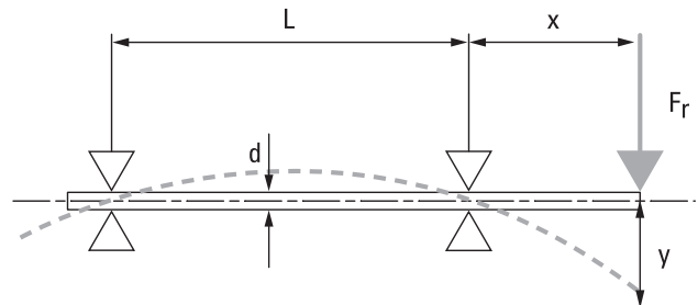
Fig. 25. Deflection of the bare spindle on two supports.
