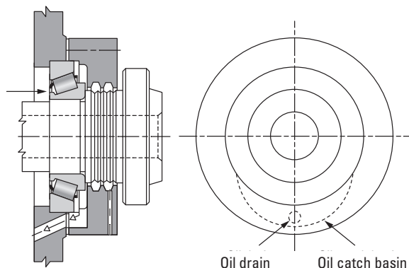
Fig. 61. Oil drain design.
