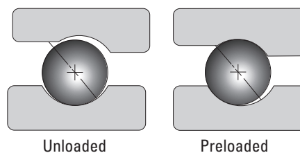
Fig. 7. Effect of preloading on ball bearing raceway contact.
