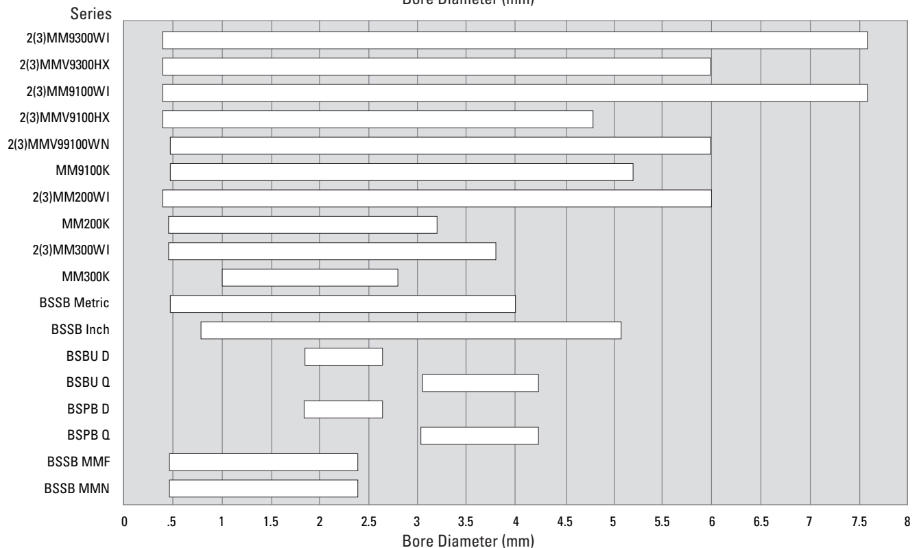
Fig. 136. Bore diameters.
