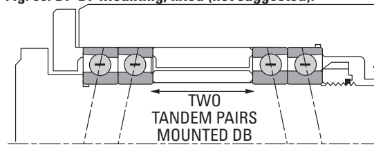
Fig. 90. DF-DF Mounting, fixed (not suggested).
