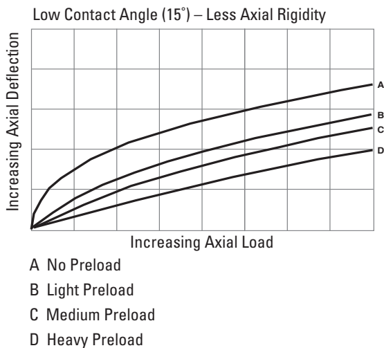
Fig. 18. Effect of contact angle on axial deflection.
