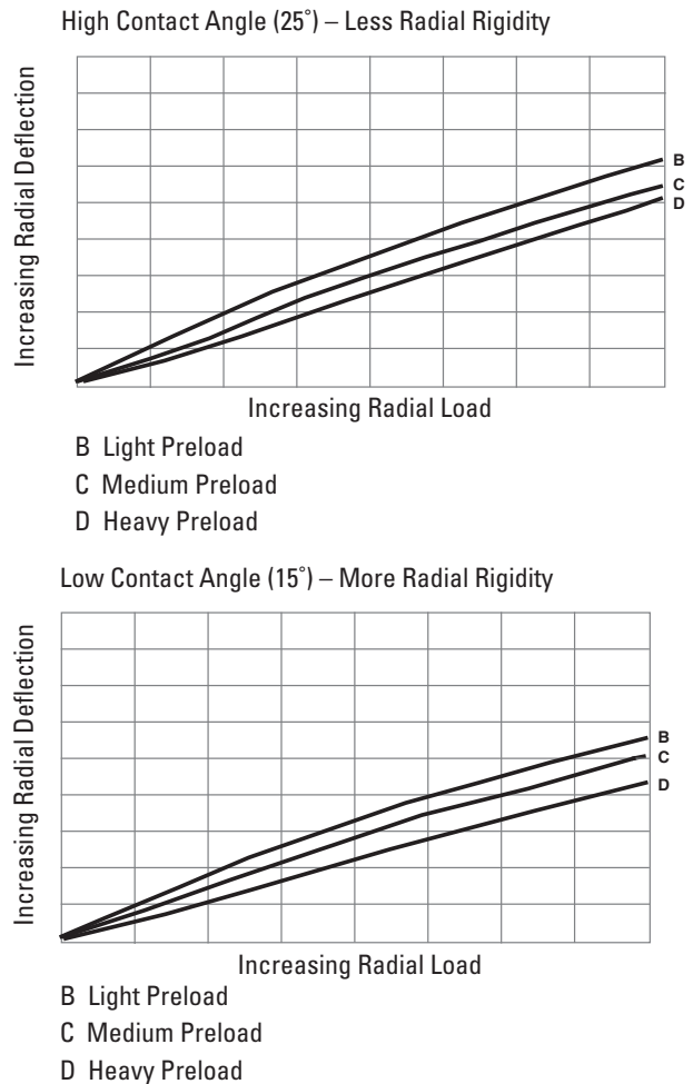
Fig. 19. Effect of contact angle on radial deflection.
