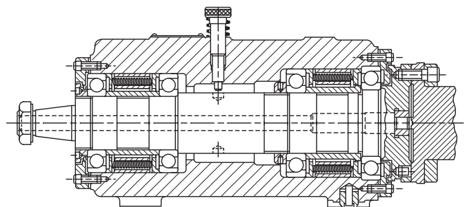
Fig. 127. High-speed precision-boring head.
