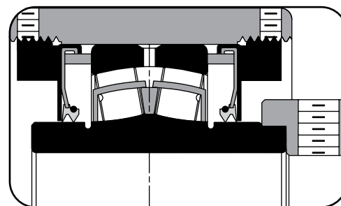
Fig. 15. Double-lip seals.
