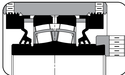
Fig. 13. Triple-lip seals.
