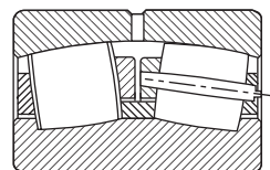
Fig. 8. Pin-type cage.
