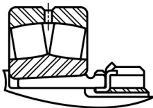
Fig. 13. Mounting with withdrawal sleeve
