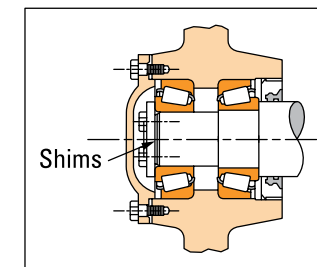
Figure 23. End Plate
