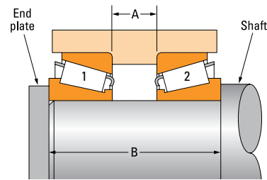
Figure 7. Machine Assembly
