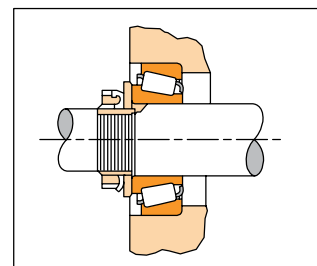
Figure 21. Locknut
