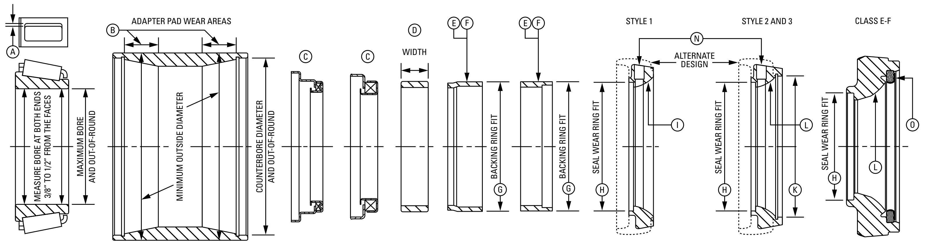
ROLLER ASSEMBLY OUTER RING (CUP) ECOTURN® SEAL HDL™ SEAL SPACER SEAL WEAR RING HDL™ SLEEVE NON-FITTED BACKING RINGS FITTED BACKING RINGS SURE-FIT® BACKING RING
