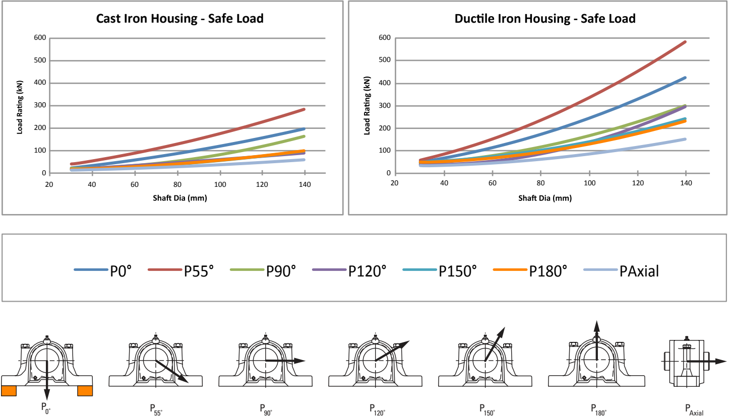
Figure 7: comparison of housing safe loads for both cast iron and ductile iron.
