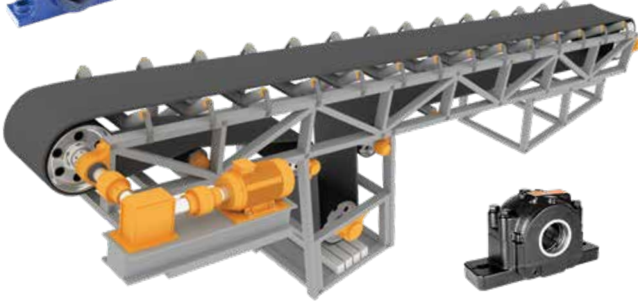
Timken® SAF/SNT mounted split-block spherical roller bearing
