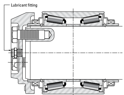
Fig. 39 Mounting Arrangement 3
