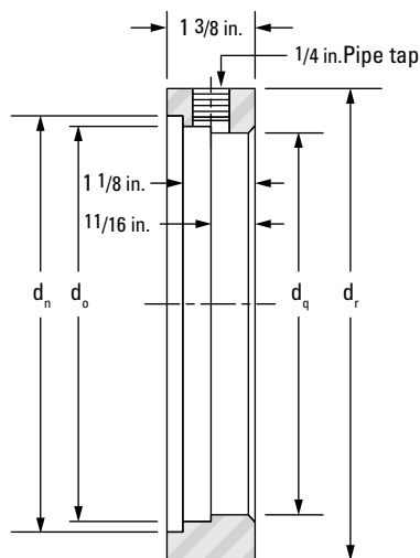
Backing Spacer
