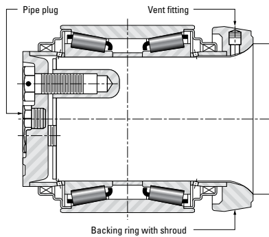
Fig. 49 Mounting Arrangement 6
