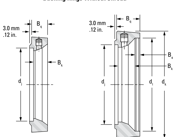
Backing Rings Without Shroud
