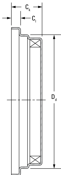
Seal Case
