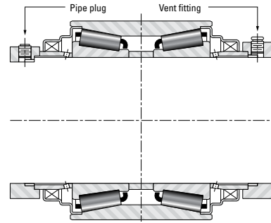
Fig. 48 Mounting Arrangement 5D
