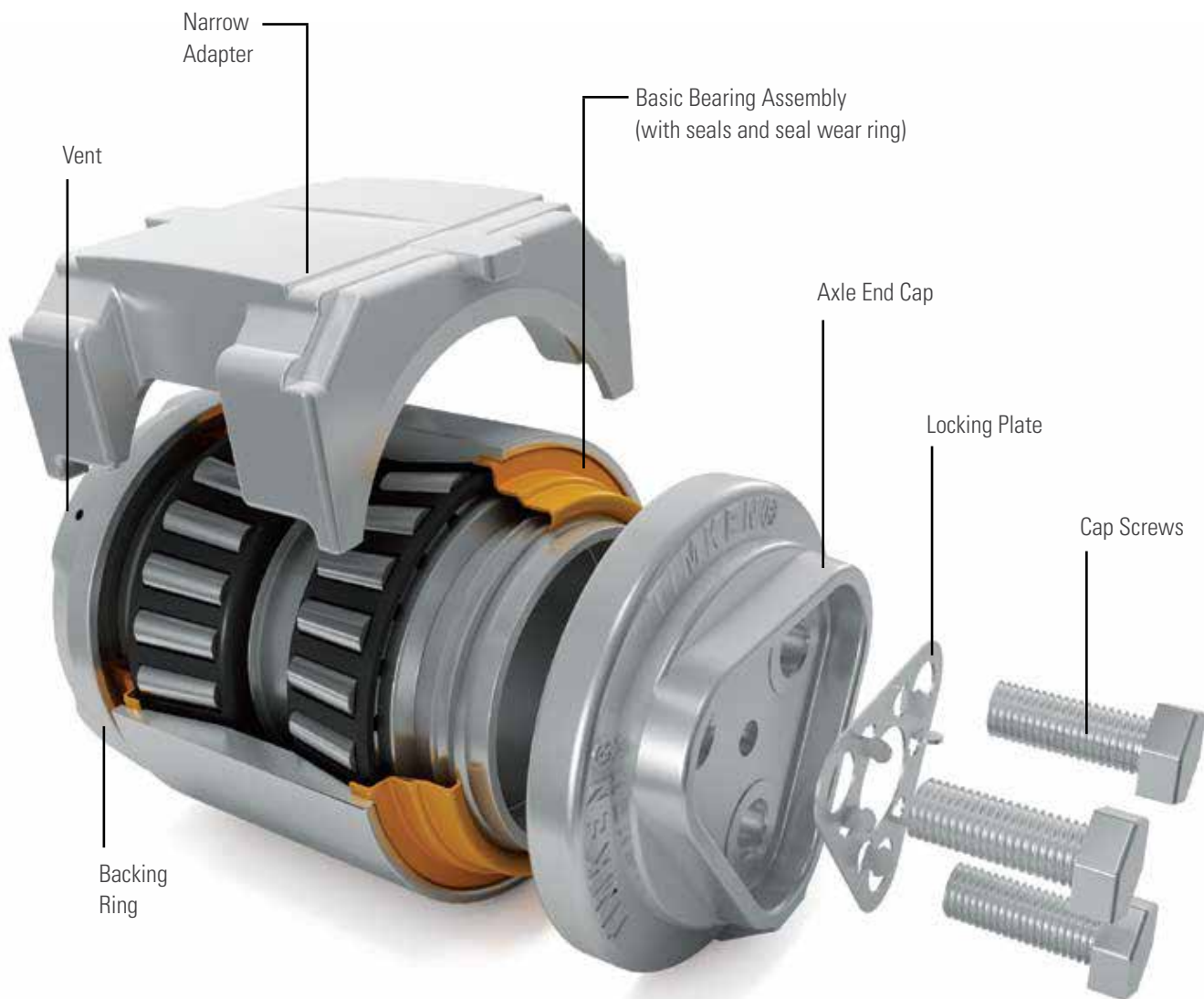
Fig. 30 3D illustration of AP bearing
