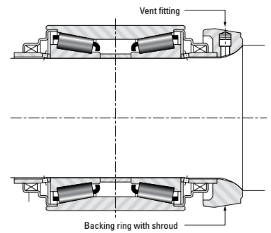
Fig. 36 Mounting Arrangement 2
