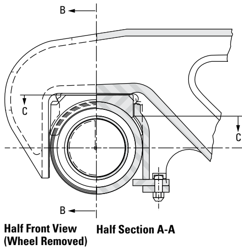
Fig. 19 Mounted adapter
